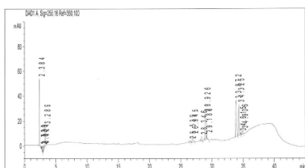
Figure 2: Chromatogram of sample 2 (Source: DATU Laboratory).
