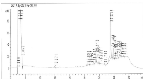
Figure 3: Chromatogram of sample 3 (Source: DATU Laboratory).
