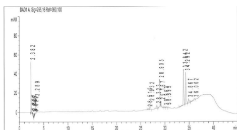
Figure 5: Chromatogram of sample 5 (Source: DATU Laboratory).
